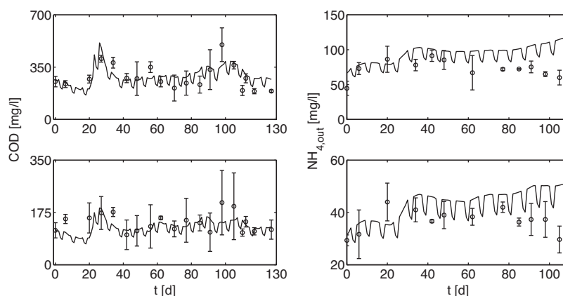
Fig. 2. Comparison between COD (left panels) and NH_4^+ (right panels) effluent concentrations simulated (continuous line) and measured (circle with standard deviation bar) for group A (upper panels) and B (lower panels).
