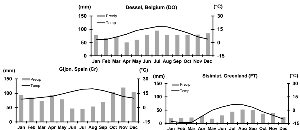
Fig. 2 Climatographs of Dessel (DO), Gijon (Cr) and Sisimiut (FT) analogue stations.
