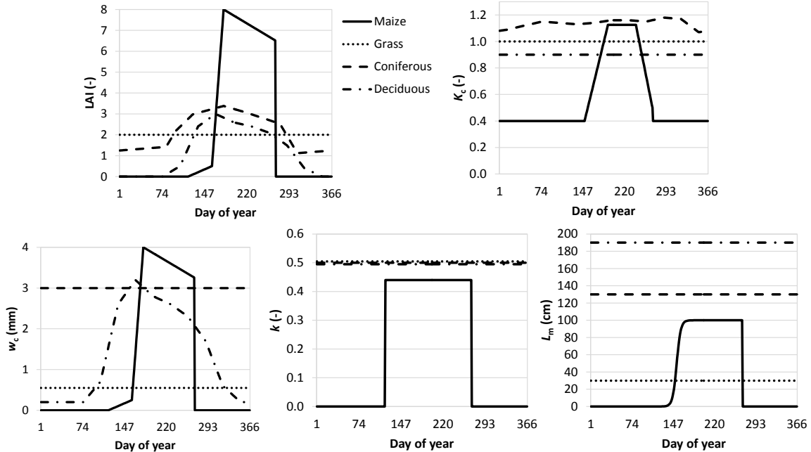
Fig. 3 Daily variability of vegetation parameters used for the modelling of potential evapotranspiration and groundwater recharge. LAI: leaf area index (grass: Jacques et al. (2011), coniferous: Vincke & Thiry (2008), deciduous: Lawrence (pers.comm.) based on Lawrence & Slingo (2004)); K_c : crop coefficient (maize: Allen et al. (1998), coniferous: Meiresonne et al. (2003) based on Gellens-Meulenberghs & Gellens (1992), deciduous: City of Riverside Planning Department (1994) cited in Amador et al. (2007)); w_c : interception capacity (maize: w_c = \text{LAI} \times 0.5 so that mean interception fraction ( f_{\text{int}} ) is equal to 0.10, grass: w_c = 0.55 mm so that f_{\text{int}} = 0.15 (Meyus et al. , 2004), coniferous: Breuer et al. (2003), deciduous: w_c (mm) = LAI+0.2 so that mean f_{\text{int}} = 0.15 (Breuer et al. , 2003)); k : light extinction coefficient (maize: Flénet et al. (1996), grass: Jacques et al. (2011), coniferous and deciduous: Granier et al. (1999); L_m : maximum root depth (grass: Jacques et al. (2011), coniferous: Vincke & Thiry (2008), deciduous: Breuer et al. (2003)).
