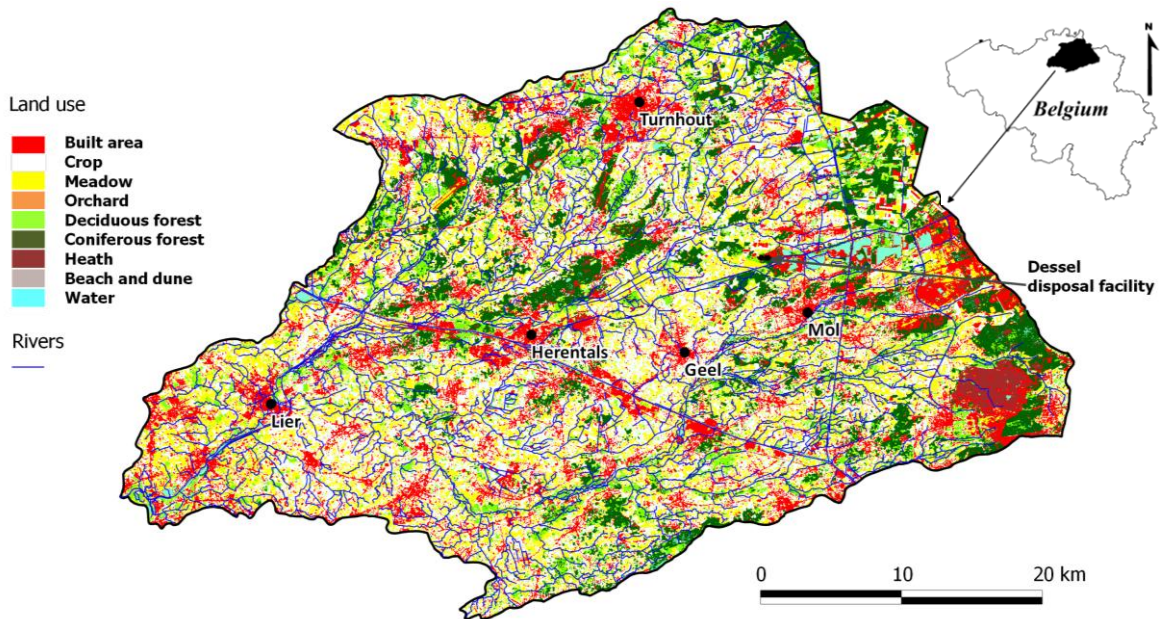
Fig. 1 Land use in the Nete catchment (source: Landsat 2001 supervised classification; AGIV, 2011).
