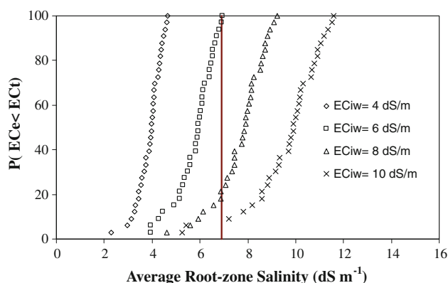
Fig. 11 The probability distribution function of the root-zone salinity ( EC_e ) being smaller than the wheat yield threshold ( EC_t ) obtained by simulating the 33-year series with irrigation waters of an EC_{iw} of 4, 6, 8, and 10 dS\ m^{-1}
