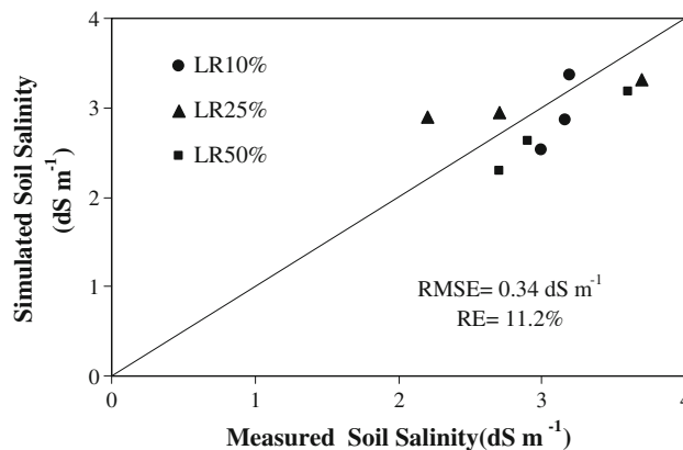
Fig. 2 Comparison between measured and simulated (with the UNSATCHEM model) soil salinities for experimental treatments with irrigation water with salinity of 2.5 \text{ dS m}^{-1} and three different leaching requirements (LR 10 %, LR 25 %, and LR 50 % are leaching requirements for 10, 25, and 50 % yield reductions, respectively)
