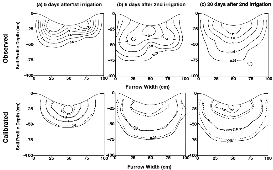
Figure 7. Measured and calibrated solute concentrations in plot 1 at different soil sampling times (dashed lines = CDE, and continuous lines = MIM).
