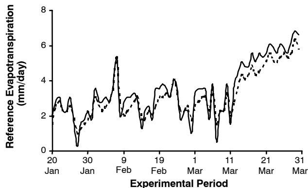
Figure 2. Reference pan evapotranspiration rates and rates estimated using the Penman-Monteith method (dashed line = Penman-Monteith, and continuous line = pan).
