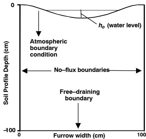
Figure 4. Applied water and solute boundary conditions for the specified soil profiles.
