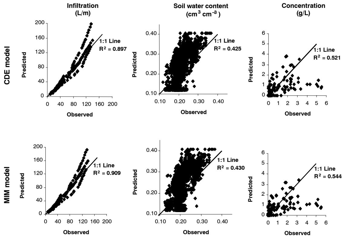
Figure 5. Measured versus predicted (using the CDE and MIM transport models) cumulative infiltration rates, soil water contents, and solute concentrations for all experimental plots.
