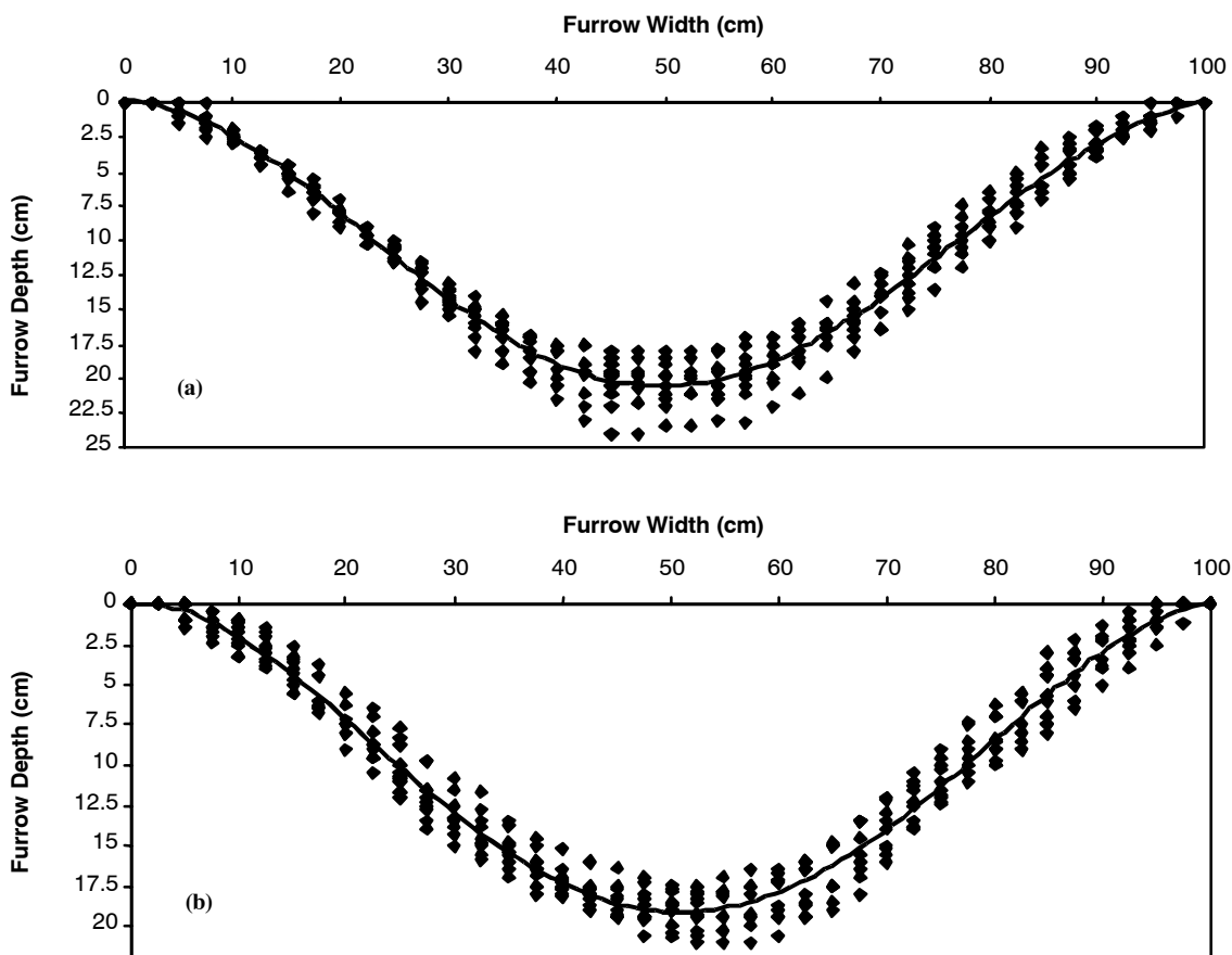
Figure 1. Geometries of the experimental furrows and the fitted profiles. Symbols are the measured data and solid lines are the best fits: (a) before the first irrigation, and (b) before the second irrigation.
