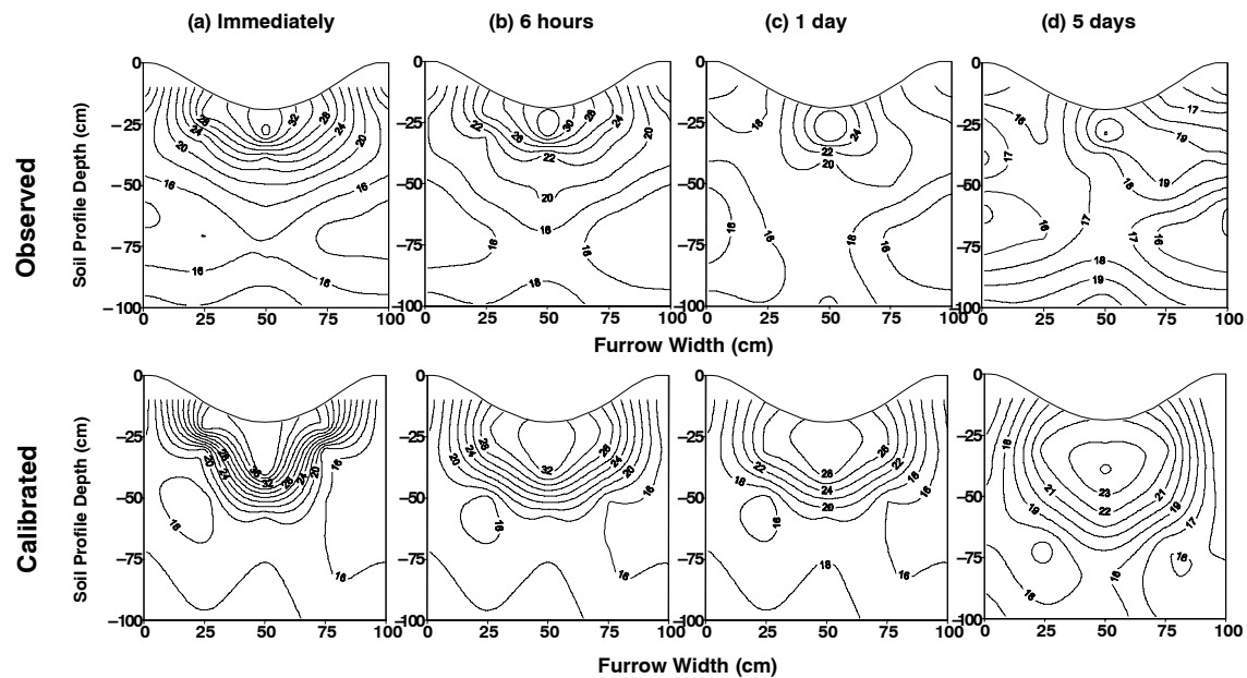
Figure 6. Measured and calibrated soil water contents in plot 1 at different times after the first irrigation event.
