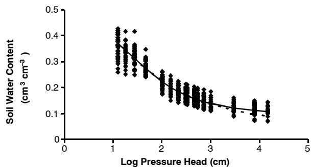
Figure 3. Measured and fitted soil water retention curves (symbols = measured, dashed line = RETC and Rosetta optimization, and continuous line = RETC optimization).
