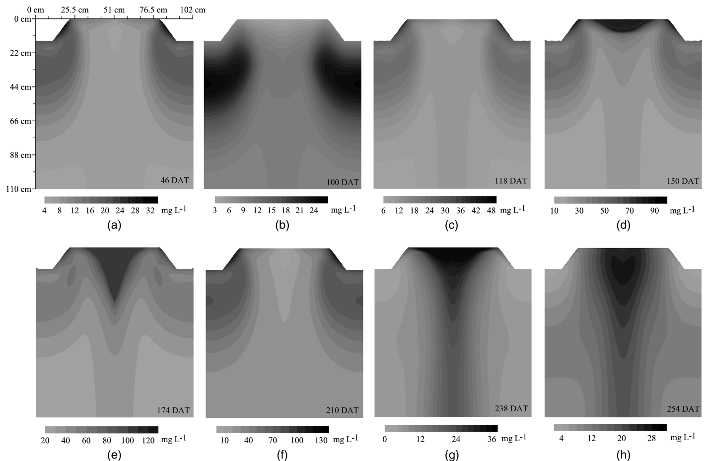
Fig. 5. Simulated spatial distributions of nitrate-nitrogen ( \text{NO}_3\text{-N} ) concentrations within the flow domain at different times during the onion growing season: (a and b) on 46 DAT (days after transplanting) and 100 DAT of the establishment stage of onion growth; (c and d) on 118 DAT and 150 DAT of the development (vegetative) and early stage of bulb formation; (e) on 174 DAT of the bulb formation and bulb growth stage; (f and g) on 210 DAT and 238 DAT of the bulb enlargement or maturity stage; (h) on 254 DAT prior to the harvest on 255 DAT
